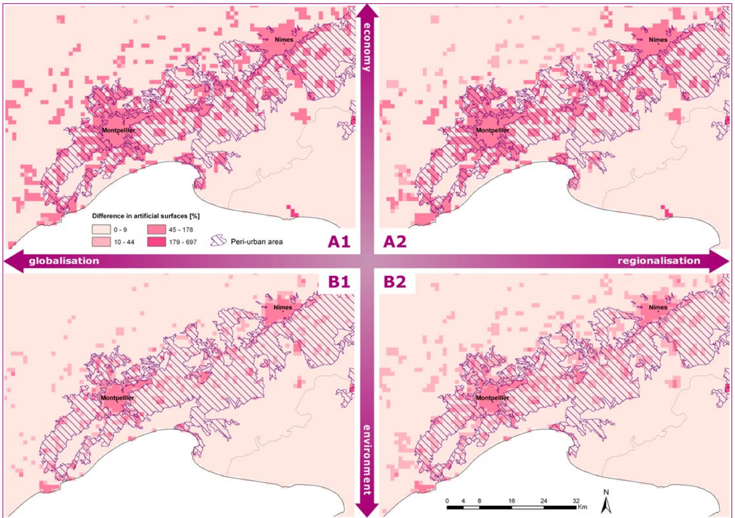
Difference in artificial surfaces, as a percentage of the current coverage, in the Montpellier region by 2025 for scenarios A1-hyper-tech, A2-extreme water, B1-peak oil and B2-fragmentation. The hatching shows the areas classed as peri-urban.
